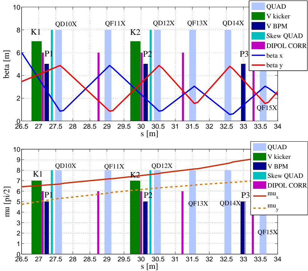
Figure 1: Layout of the region of the extraction line of the ATF2 optics version 3.8 where the FONT elements are located: kickers K1 and K2, and BPMs P1, P2 and P3. Top: transverse betatron functions \beta_{x,y} . Bottom: transverse phase advance functions \mu_{x,y} .
