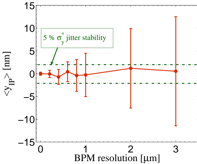
Figure 4: Vertical jitter at the IP versus BPM resolution.
