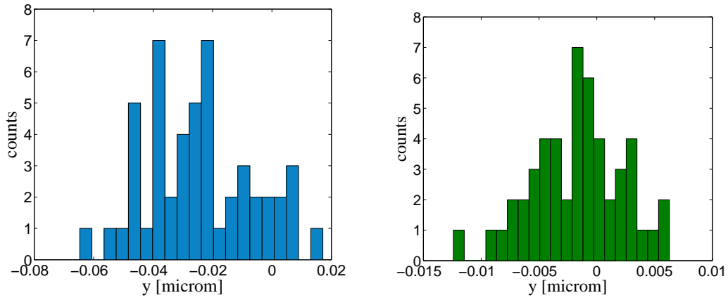
Figure 3: Jitter distribution at the IP, before steering correction (left) and after steering correction (right).
