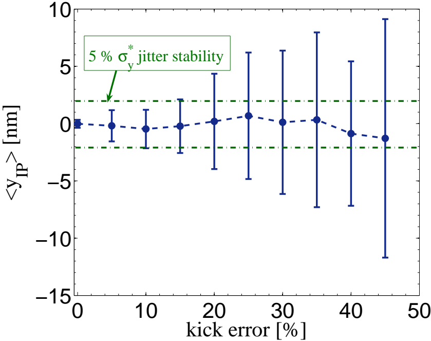
Figure 5: Vertical jitter at the IP versus the kicker jitter error.
