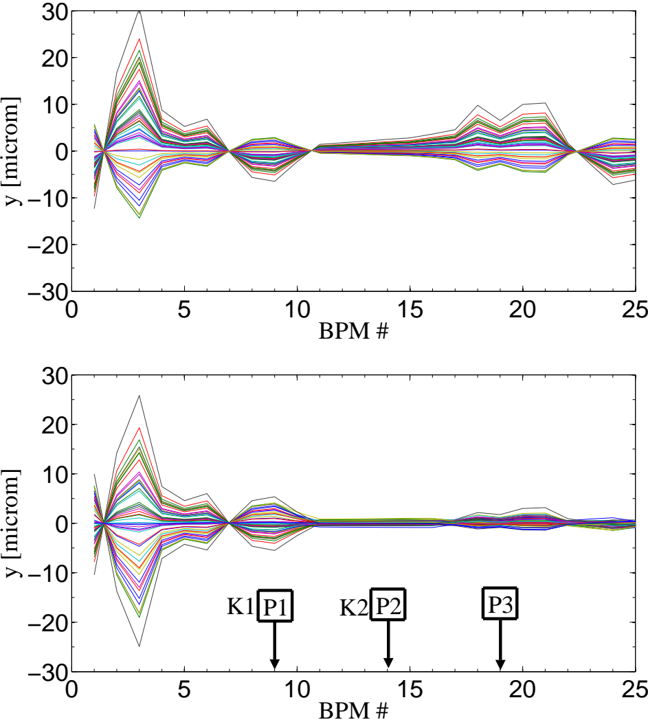
Figure 2: Jitter propagation along the ATF2 extraction region. Top: before correction. Bottom: after orbit steering correction by the kickers K1 and K2.
