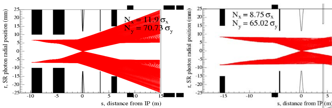
Fig. 4: Collimation depths for 14 mrad {L*=3.51m, SiD detector} & 2mrad (L*=4.5m, LDC).
