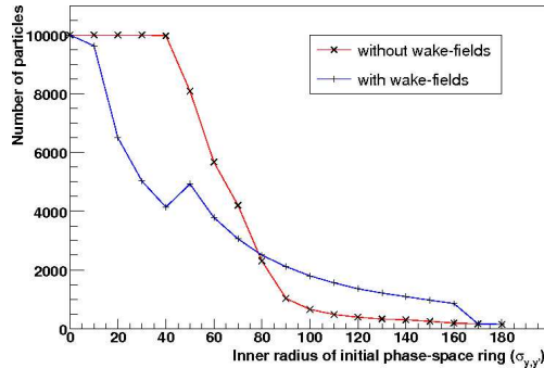
Figure 5: Number of halo particles at the IP vs inner radius of the initial phase-space ring in y, y' . Particles have an initial position within a ring of 0-5 \sigma in x, x' , and each y, y' ring has a width of 10 \sigma
