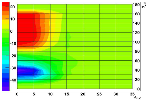
Figure 4: Significance of the difference in number of halo particles at the IP vs the inner radii of the phase-space rings from which the particles originated, in units of \sigma_{i,i'} . The ring in x, x' phase space has a width of 5 \sigma , and that of the y, y' phase-space has a width of 10 \sigma .
