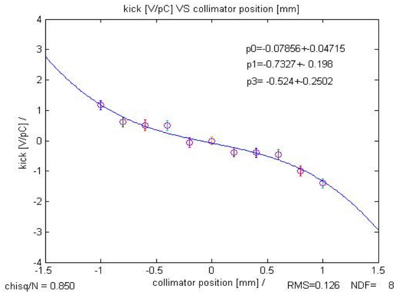
Figure 5: Collimator 6.
