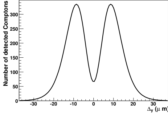
Figure 14: Scan profile at the laser-wire IP for a laser with M^2=1.3 and wavelength 532 nm operating in the TM_{01} mode and focused using f_1 optics. The electron bunch is assumed to have a Gaussian profile of \sigma_{ey} = 5 \mu\text{m} , \sigma_{ex} = 50 \mu\text{m}
