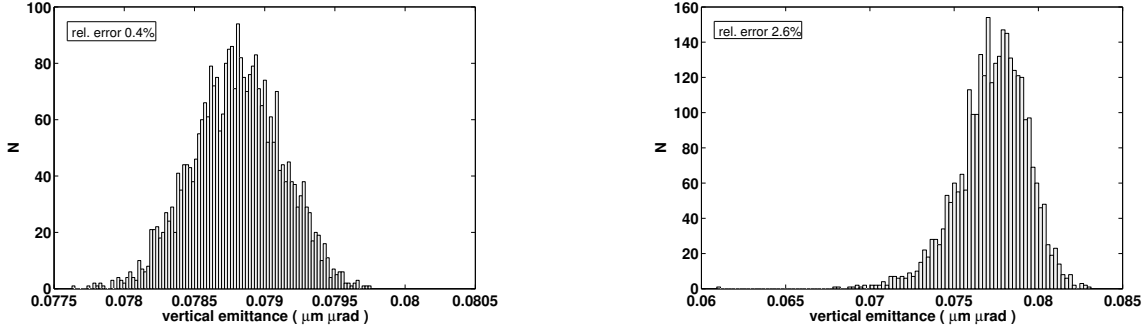
Figure 3: Distribution of reconstructed vertical emittance with 1% (a) and 5% (b) random errors on the beam size measurement for a 4d diagnostics section (statistics corresponding to train length). Initial optical functions are perfectly matched. The true emittance is 0.079 \mu\text{m} \cdot \mu\text{rad} [1].
