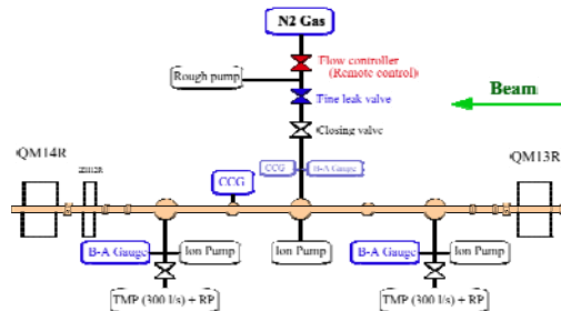
Fig. 5: Schematics of gas inlet system.
