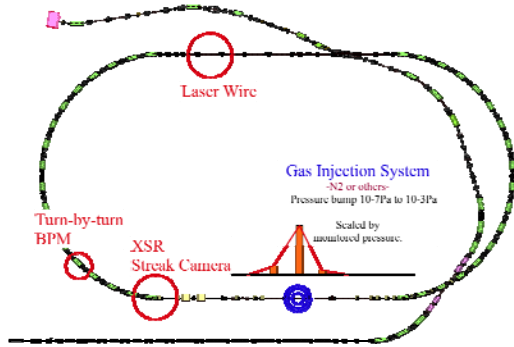
Fig. 4: Layout of devices for the fast ion study.
