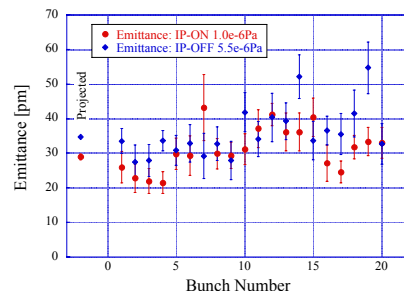
Fig.3: Emittance of multi-bunch at 20mA/20 bunches.
