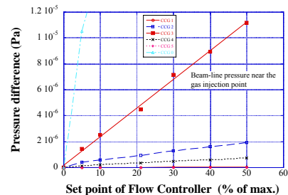
Fig.7: Vacuum pressure near the gas inlet system.
