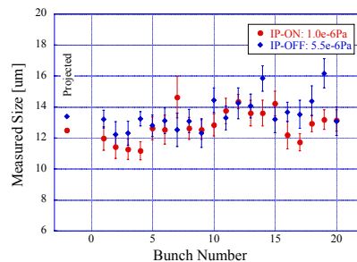
Fig.2: Measured size of multi-bunch at 20mA/20 bunches.
