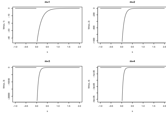
Figure 1: Transverse \delta wakes suggested by Raimondi et al
