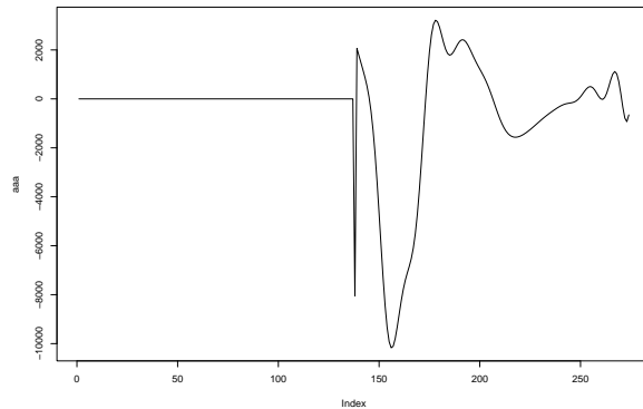
Figure 5: Reconstructed causal W_{\delta}^1
