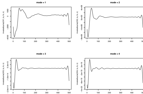
Figure 4: Reconstructed \delta wakes with \gamma = 10
