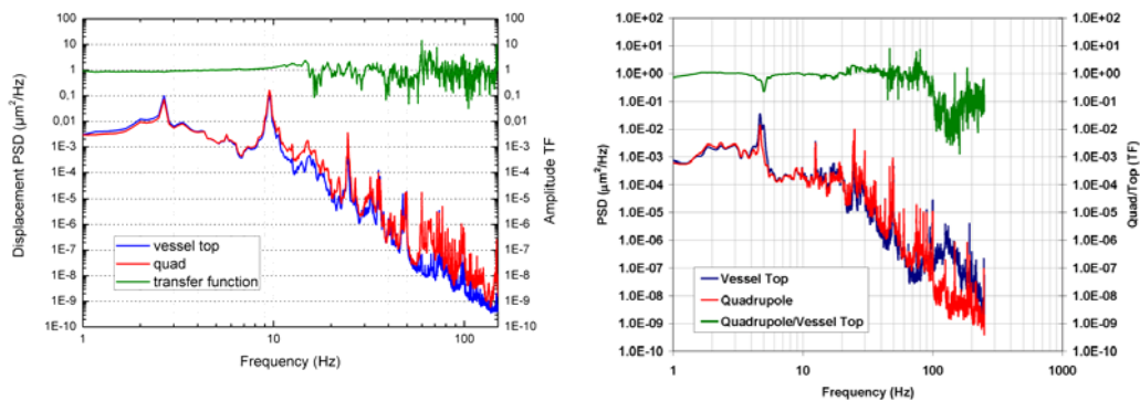
Figure 1: Quad vs.vessel top horizontal (left) and vertical (right) displacement PSDs and TFs.
