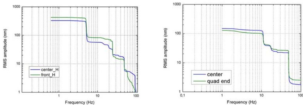
Figure 3: Quadrupole end vs. center horizontal rms comparison: inside the HeGRP with the module sitting on concrete blocks (left). On top of the vessel with Module 6 installed on the CMTB (right); in this configuration, a slightly larger amplitude was measured at the center.
