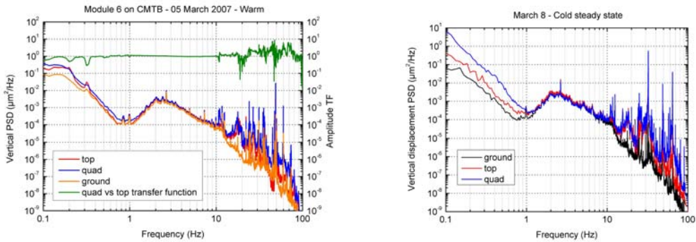
Figure 4: PSD spectra measured on the CMTB floor, on top of the vacuum vessel and on the quadrupole at room temperature (left), and in cold steady state with RF off (right).
