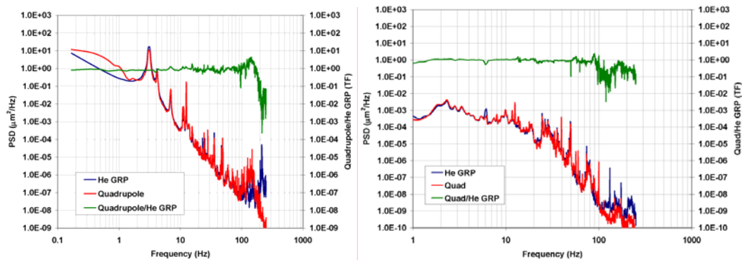
Figure 2: Quad vs. HeGRP: (left) horizontal displacement PSDs and TF measured during Module 6 assembly; the peaks below 10 Hz in the PSD are resonances of the assembly stand; (right) vertical displacement PSDs and TF measured with Module 6 on the CMTB.
