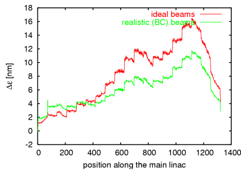
Figure 2: Emittance growth along the CLIC main linac, for a set of ideal, Gaussian, test beams (in red) vs realistic test beams obtained simulating the bunch compressor (in green), after the full alignment procedure.
