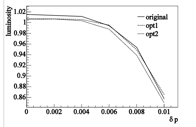
Figure 2. Geometric luminosity (normalised to the design luminosity) as a function of energy deviation for the original and optimised ILC BDS lattices.
