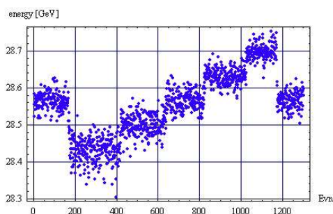
Figure 5: Energy scan as seen by the spectrometer.
