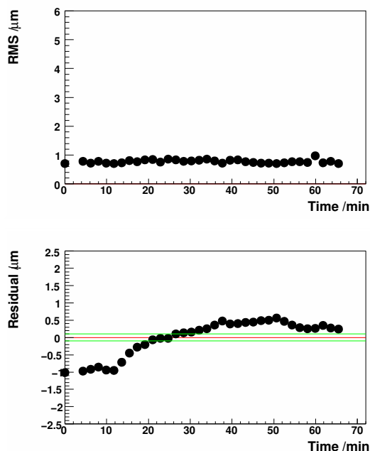
Figure 3: Precision of the BPM system over a period of 1 hour
