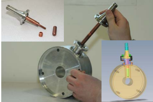
Figure 3. Prototype coupler
