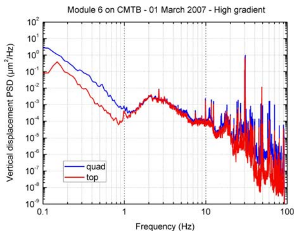
Figure 6: PSDs measured on vessel top and on quad during high power RF tests: the klystron was running at 10 Hz and the average gradient achieved was ~27 MV/m.
