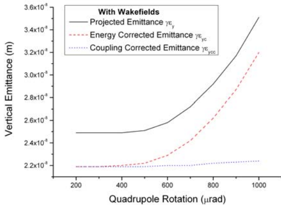
Figure 1: Vertical emittance in m after DMS as a function of the quadrupole rotation (averaged over 100 seeds). The injection emittance is \gamma_{e,y_i} = 20 \text{ nm} .
